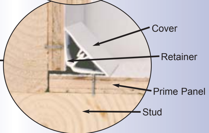
PV66-3 2 Piece Inside Corner
