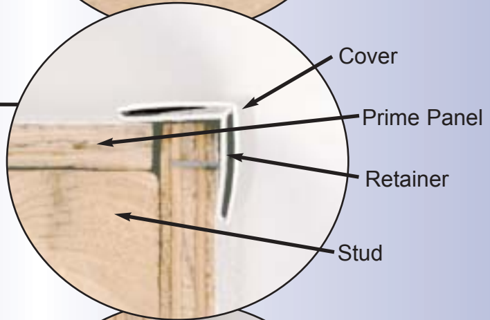
PV66-4 2 Piece Outside Corner
