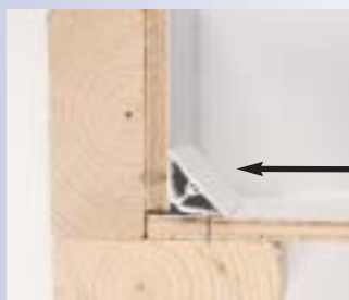
PV66-3 2 Piece Inside Corner
